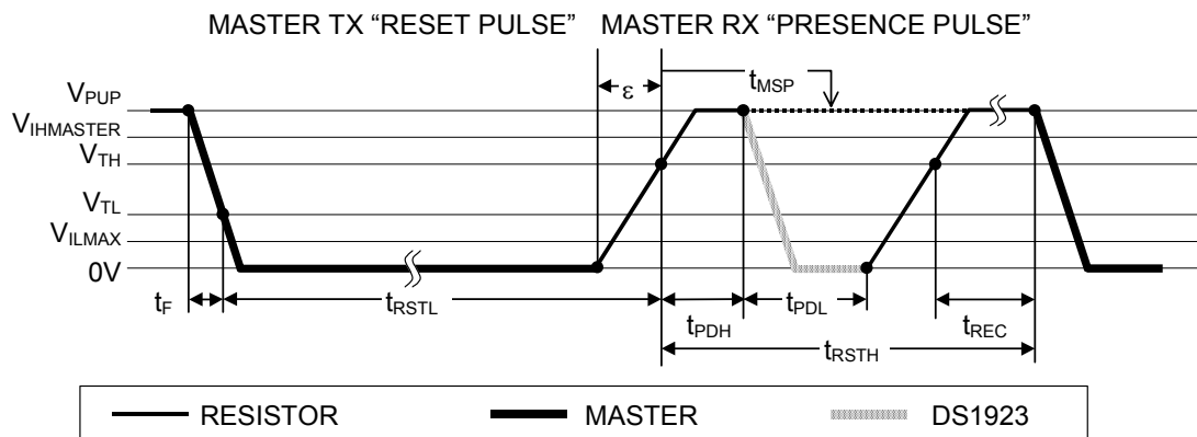
Figure 12. INITIALIZATION PROCEDURE “RESET AND PRESENCE PULSES”
