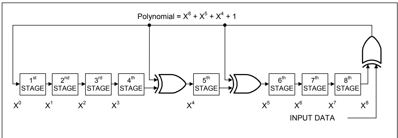
Figure 3. 1-Wire CRC GENERATOR
