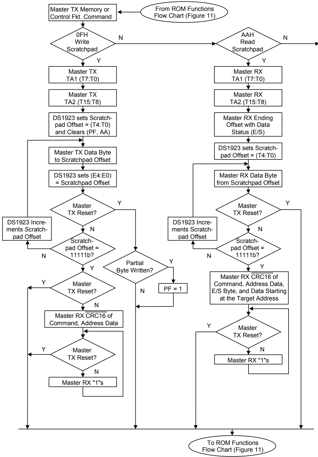
Figure 9-1. MEMORY/CONTROL FUNCTION FLOW CHART
