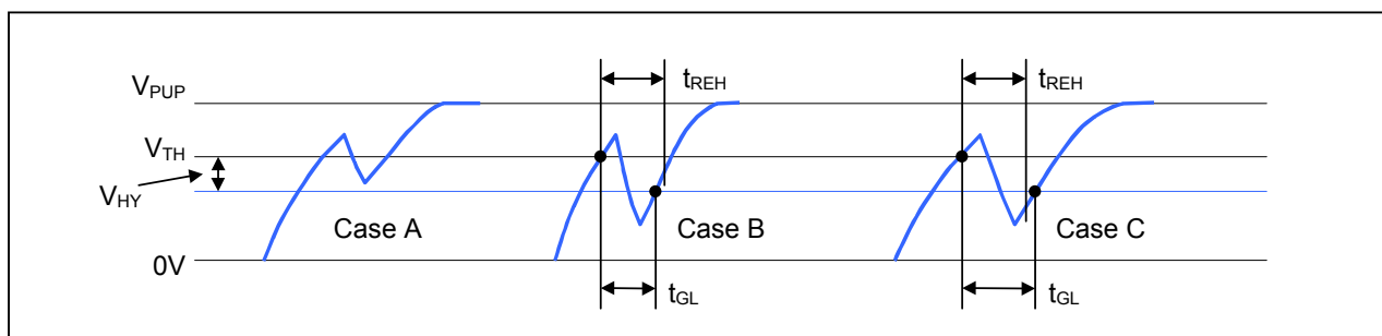
Figure 14. NOISE SUPPRESSION SCHEME
