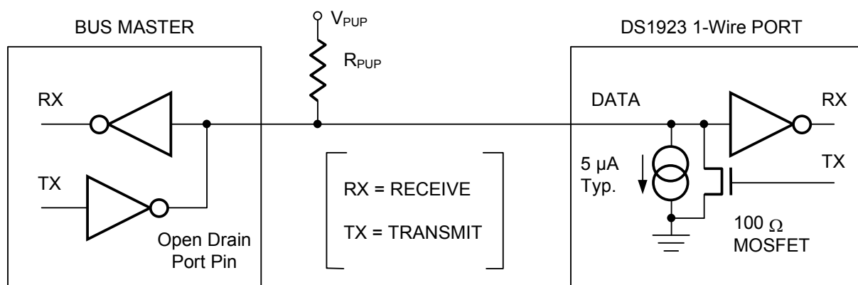
Figure 10. HARDWARE CONFIGURATION
